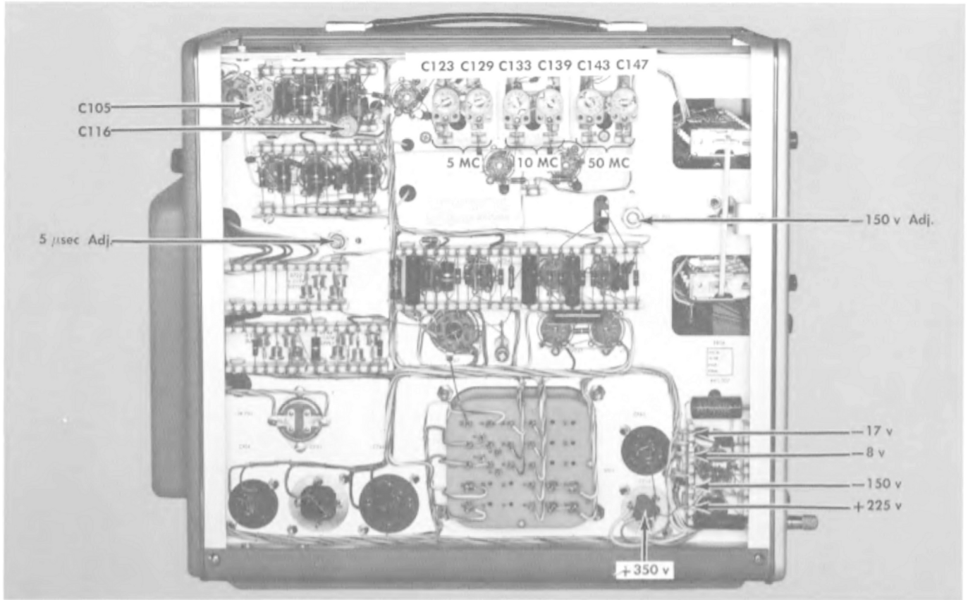
Fig. 5-3 Left side view showing voltage reading points and calibration adjustments. This covers 5/N 6386 up.
